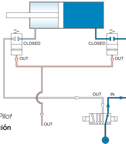
Cilindro Bloqueado Stopped Cylinder
